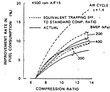
Fig. 5 Improvement Rate in Fuel Consumption with Trapping Efficiency Equivalent to Standard Compression Ratio
