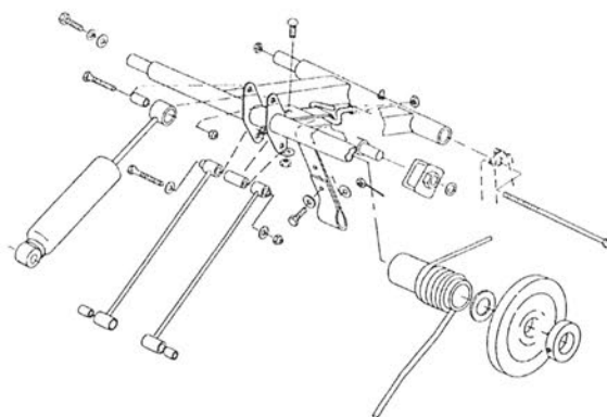
Rear Torque Arm
