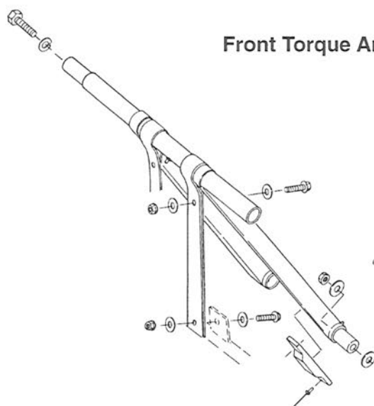
Front Torque Arm Assembly
