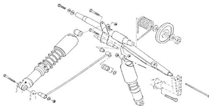
Front Torque Arm Assembly
