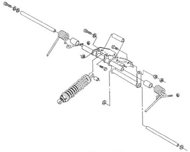
Rear Torque Arm
